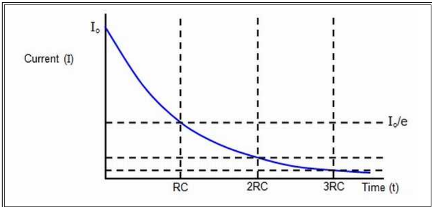
The area below the current-time curve in both charging and discharging represents the total charge held by the capacitor.
